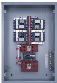
BF3-1204SDTNC
